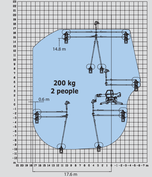
ROTATION ON STABILISERS FULLY EXTENDED WITH 3 D SYSTEM IN NEGATIVE POSITION
