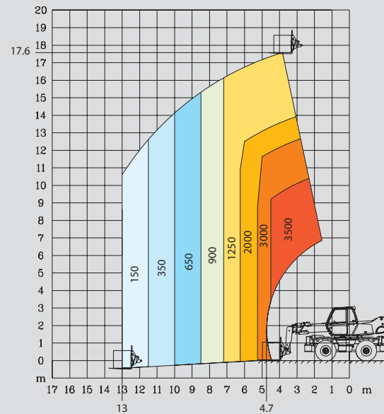
ROTATION ON STABILISERS FULLY EXTENDED WITH 4T WINCH
